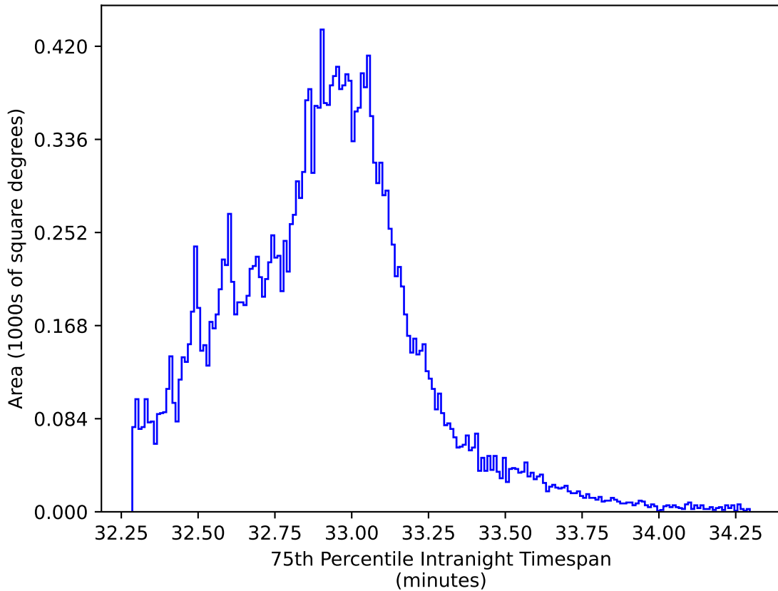
too_elab_r32_d3_griz_v3.4_10yrs All sky y band: 75th Percentile Intranight Timespan
