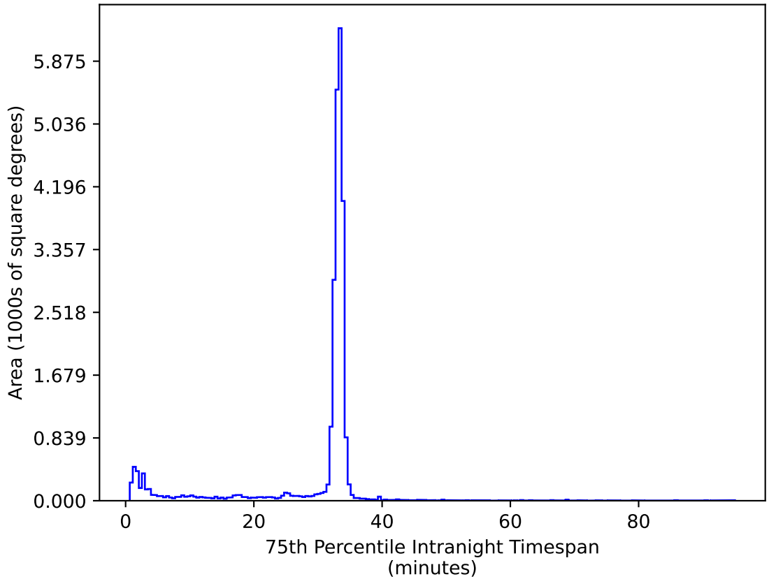
too_elab_r32_d3_griz_v3.4_10yrs All sky ug bands: 75th Percentile Intranight Timespan
