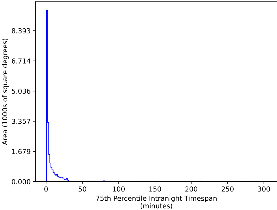
too_elab_r32_d3_griz_v3.4_10yrs All sky u band: 75th Percentile Intranight Timespan
