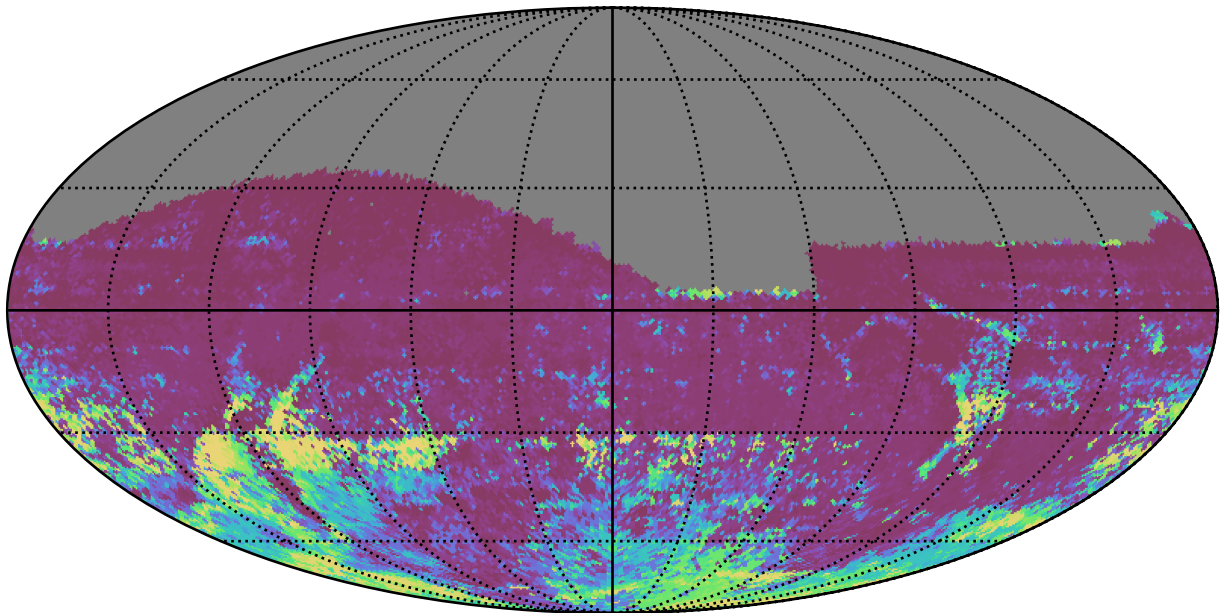
too_elab_r32_d3_griz_v3.4_10yrs All sky r band: 75th Percentile Intranight Timespan
