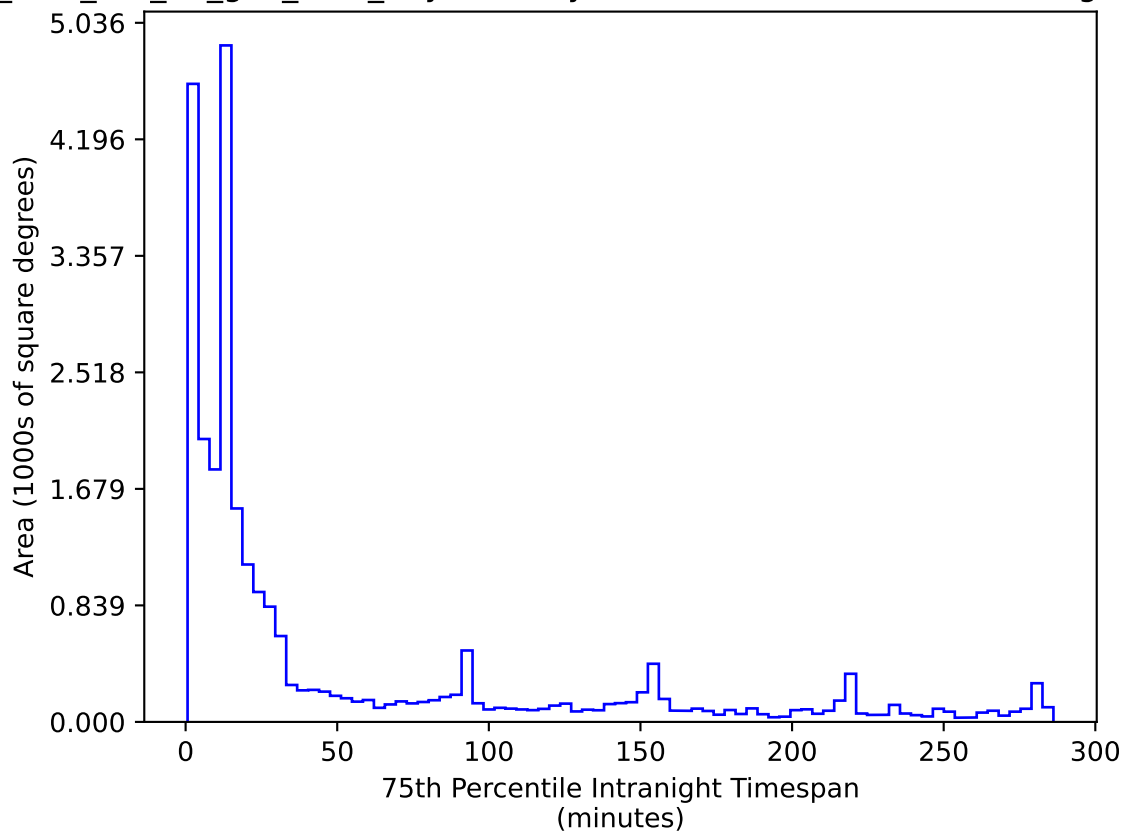
too_elab_r32_d3_griz_v3.4_10yrs All sky r band: 75th Percentile Intranight Timespan
