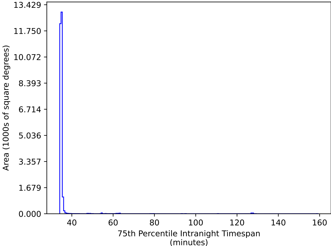
too_elab_r32_d3_griz_v3.4_10yrs All sky iz bands: 75th Percentile Intranight Timespan
