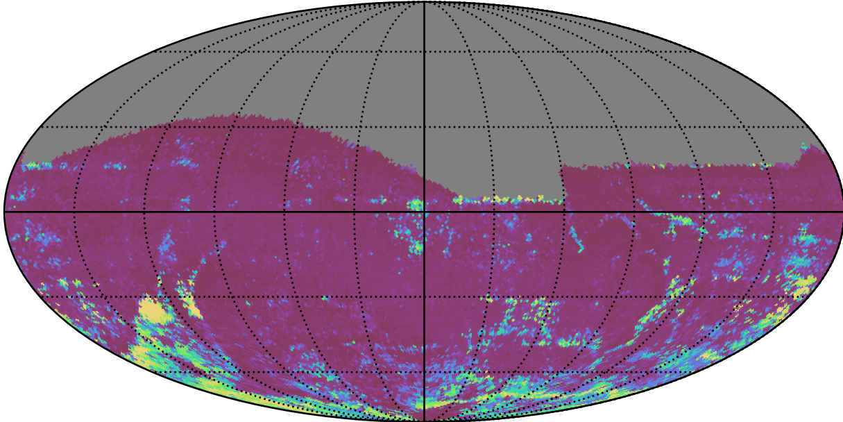
too_elab_r32_d3_griz_v3.4_10yrs All sky i band: 75th Percentile Intranight Timespan
