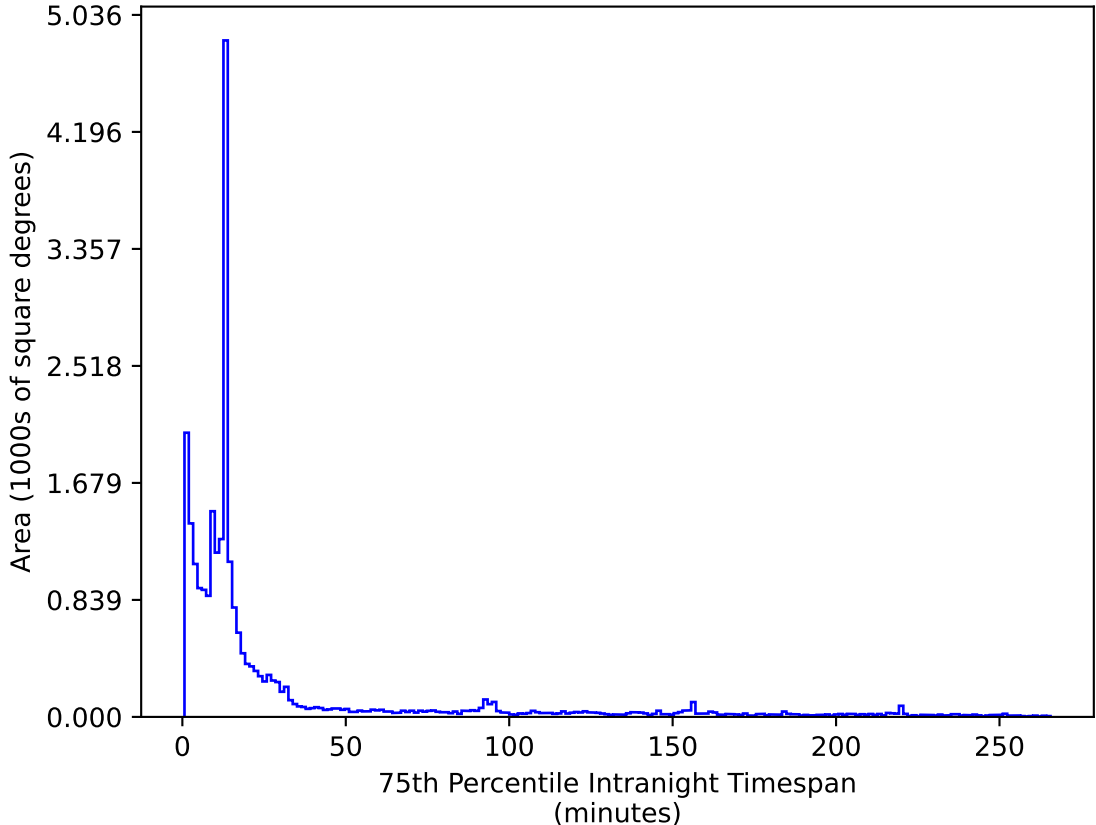
too_elab_r32_d3_griz_v3.4_10yrs All sky i band: 75th Percentile Intranight Timespan
