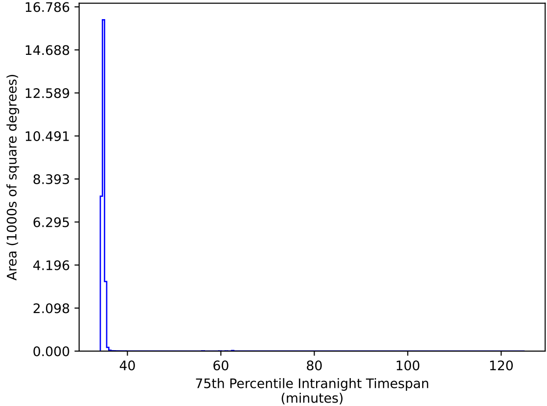
too_elab_r32_d3_griz_v3.4_10yrs All sky all bands: 75th Percentile Intranight Timespan
