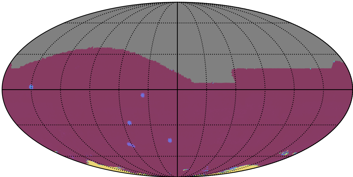
too_elab_r32_d3_griz_v3.4_10yrs All sky: 75th Percentile Intranight Timespan
