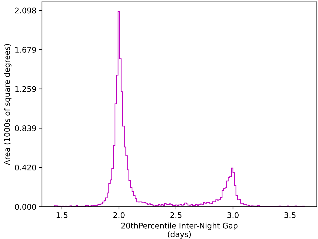
too_elab_r32_d3_griz_v3.4_10yrs WFD z band: 20thPercentile Inter-Night Gap
