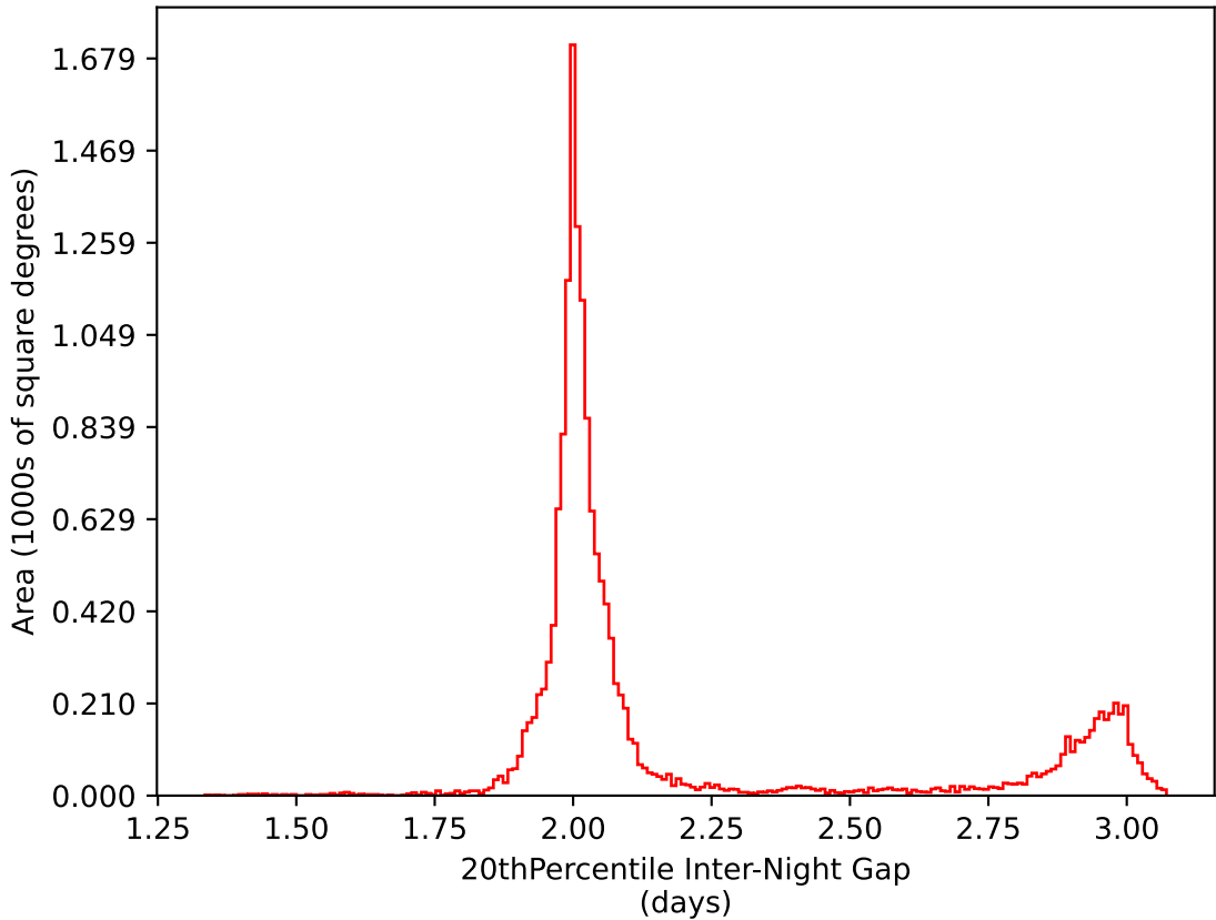
too_elab_r32_d3_griz_v3.4_10yrs WFD i band: 20thPercentile Inter-Night Gap
