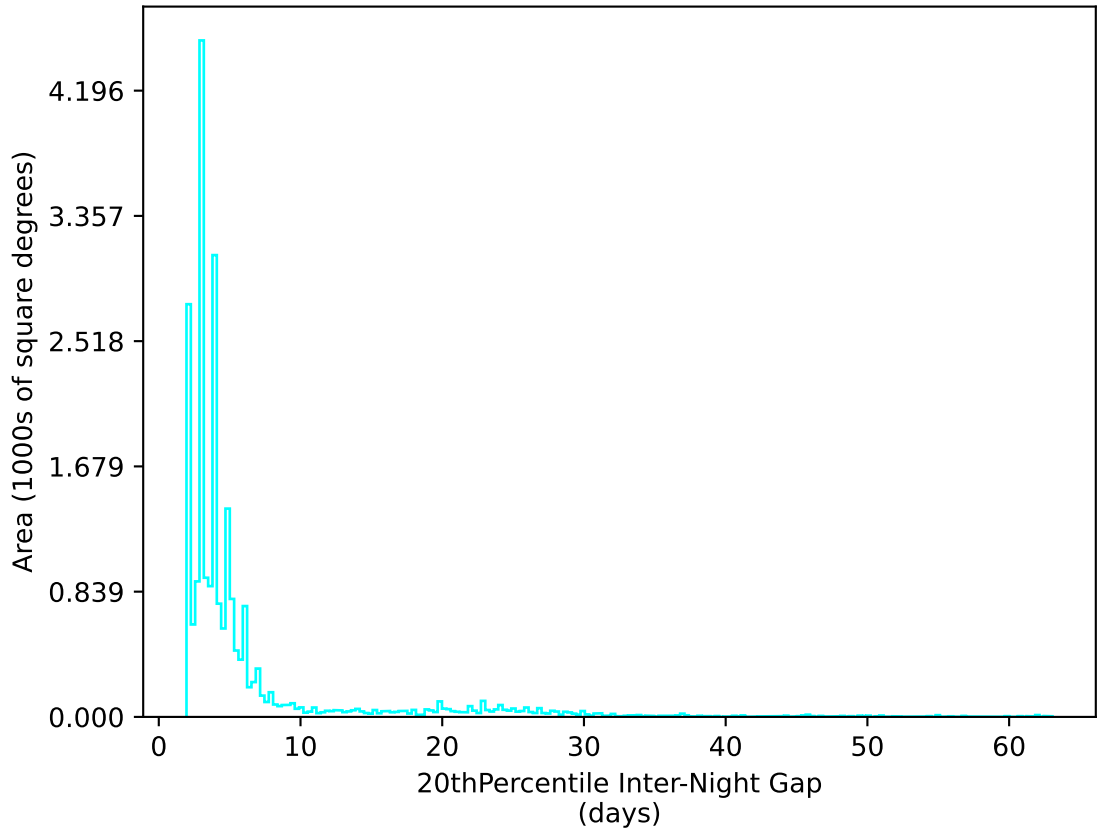
too_elab_r32_d3_griz_v3.4_10yrs All sky u band: 20thPercentile Inter-Night Gap
