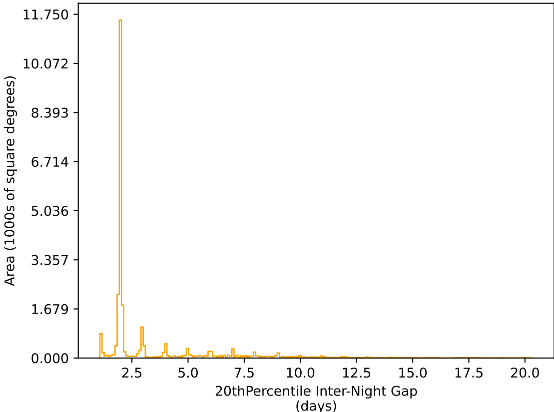
too_elab_r32_d3_griz_v3.4_10yrs All sky r band: 20thPercentile Inter-Night Gap
