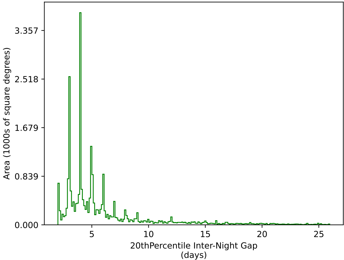
too_elab_r32_d3_griz_v3.4_10yrs All sky g band: 20thPercentile Inter-Night Gap
