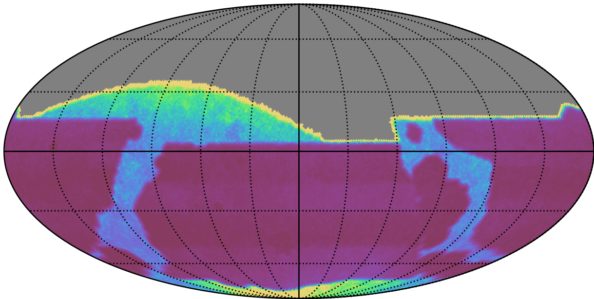
too_elab_r32_d3_griz_v3.4_10yrs : properMotion
