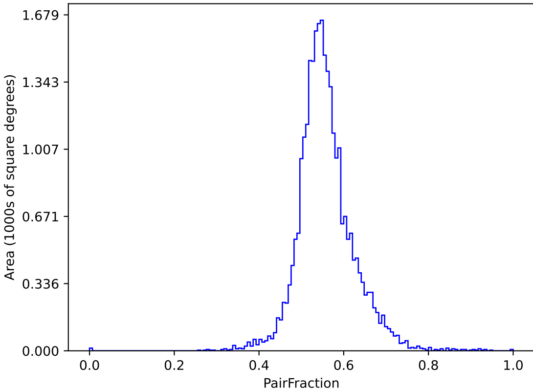
too_elab_r32_d3_griz_v3.4_10yrs (g or r or i): PairFraction
