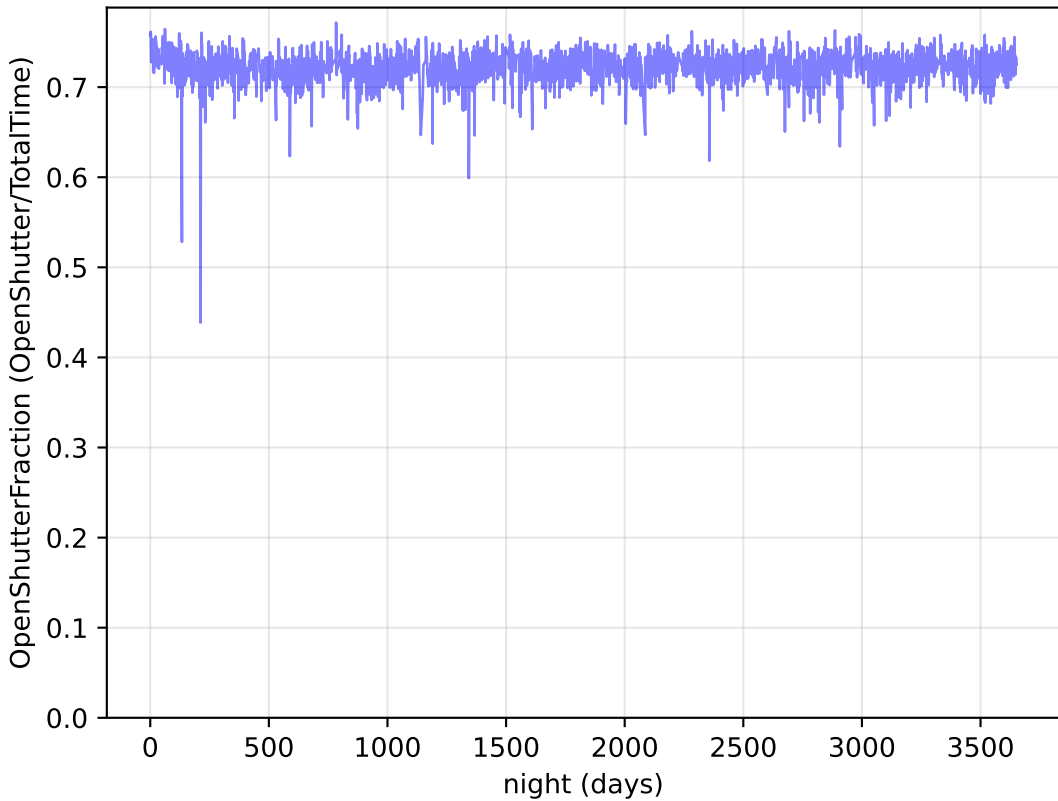
too_elab_r32_d3_griz_v3.4_10yrs : OpenShutterFraction
