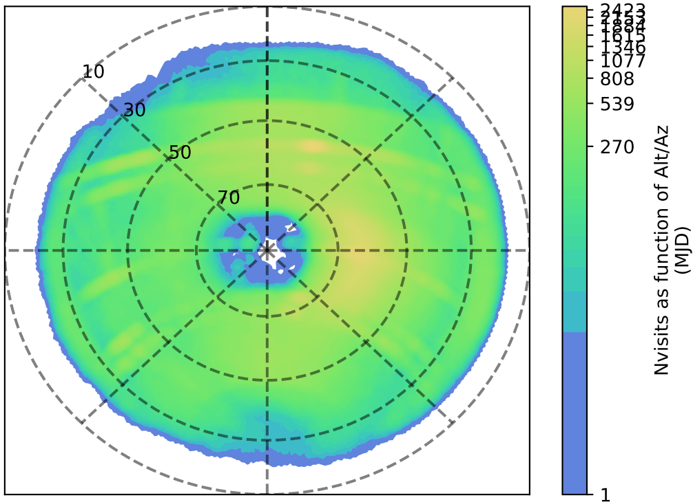
too_elab_r32_d3_griz_v3.4_10yrs z: Nvisits as function of Alt/Az
