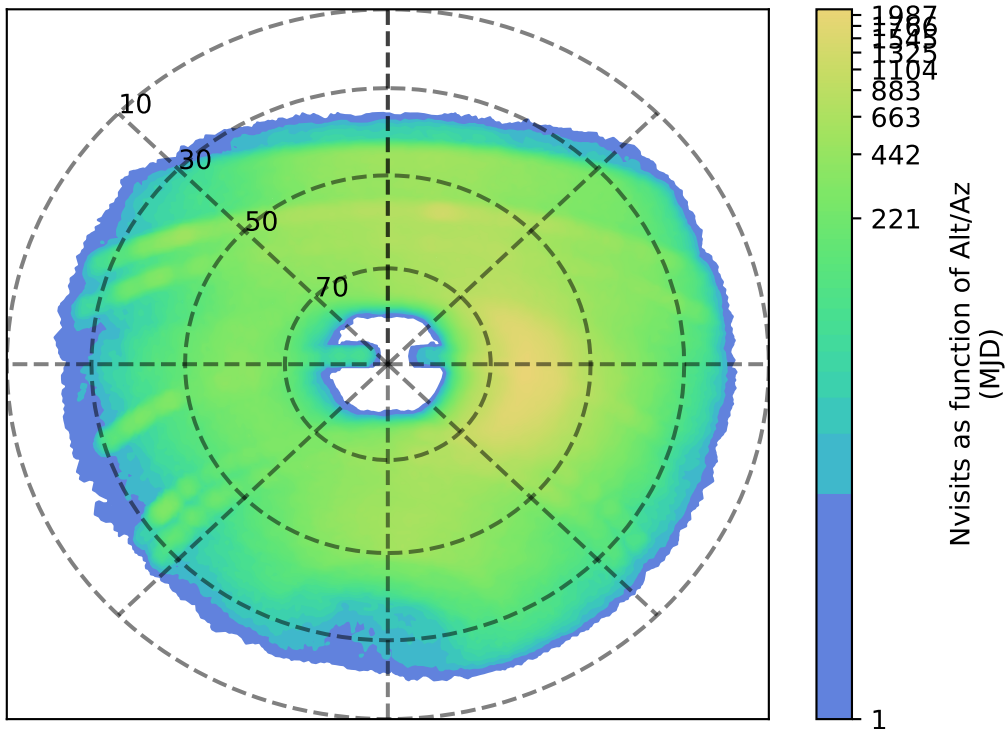
too_elab_r32_d3_griz_v3.4_10yrs y: Nvisits as function of Alt/Az
