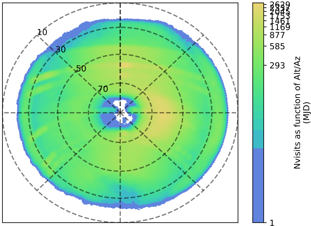
too_elab_r32_d3_griz_v3.4_10yrs i: Nvisits as function of Alt/Az
