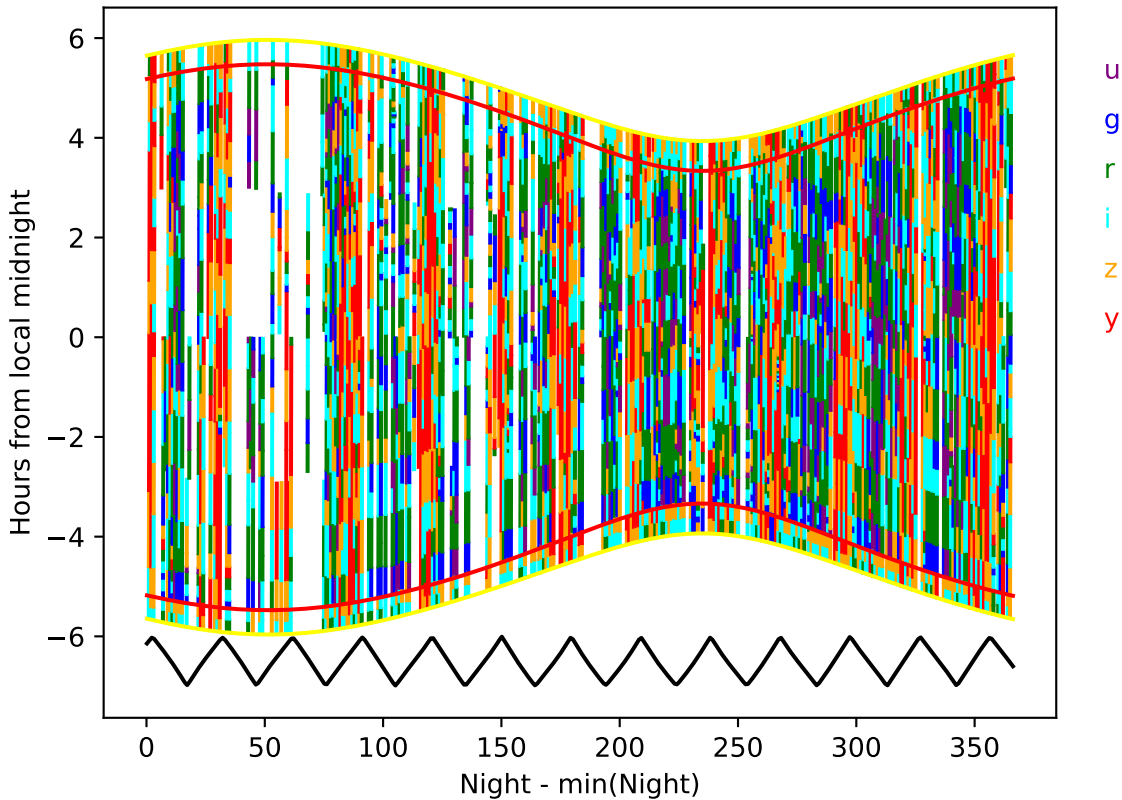
too_elab_r32_d3_griz_v3.4_10yrs year 9-10: Hourglass
