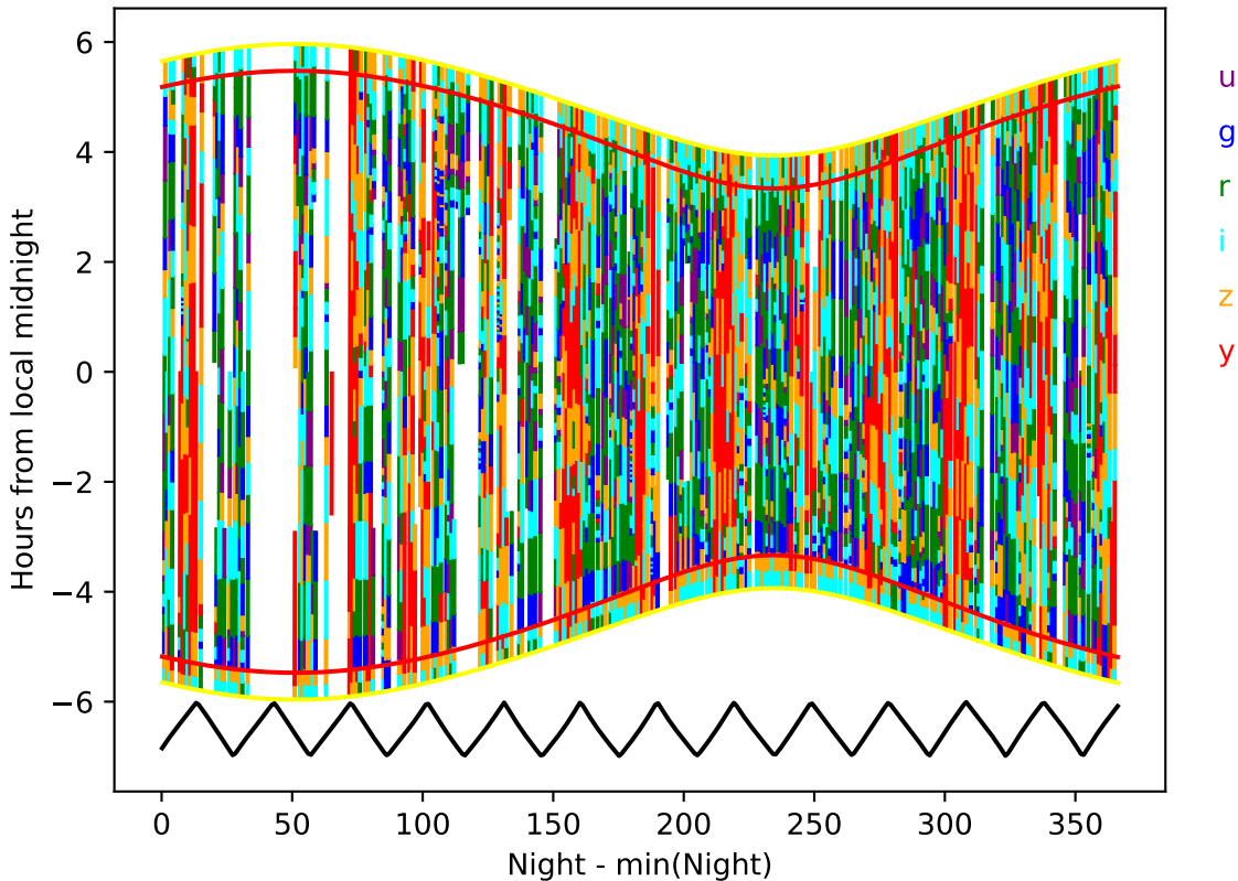
too_elab_r32_d3_griz_v3.4_10yrs year 8-9: Hourglass
