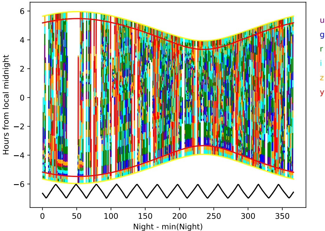
too_elab_r32_d3_griz_v3.4_10yrs year 2-3: Hourglass
