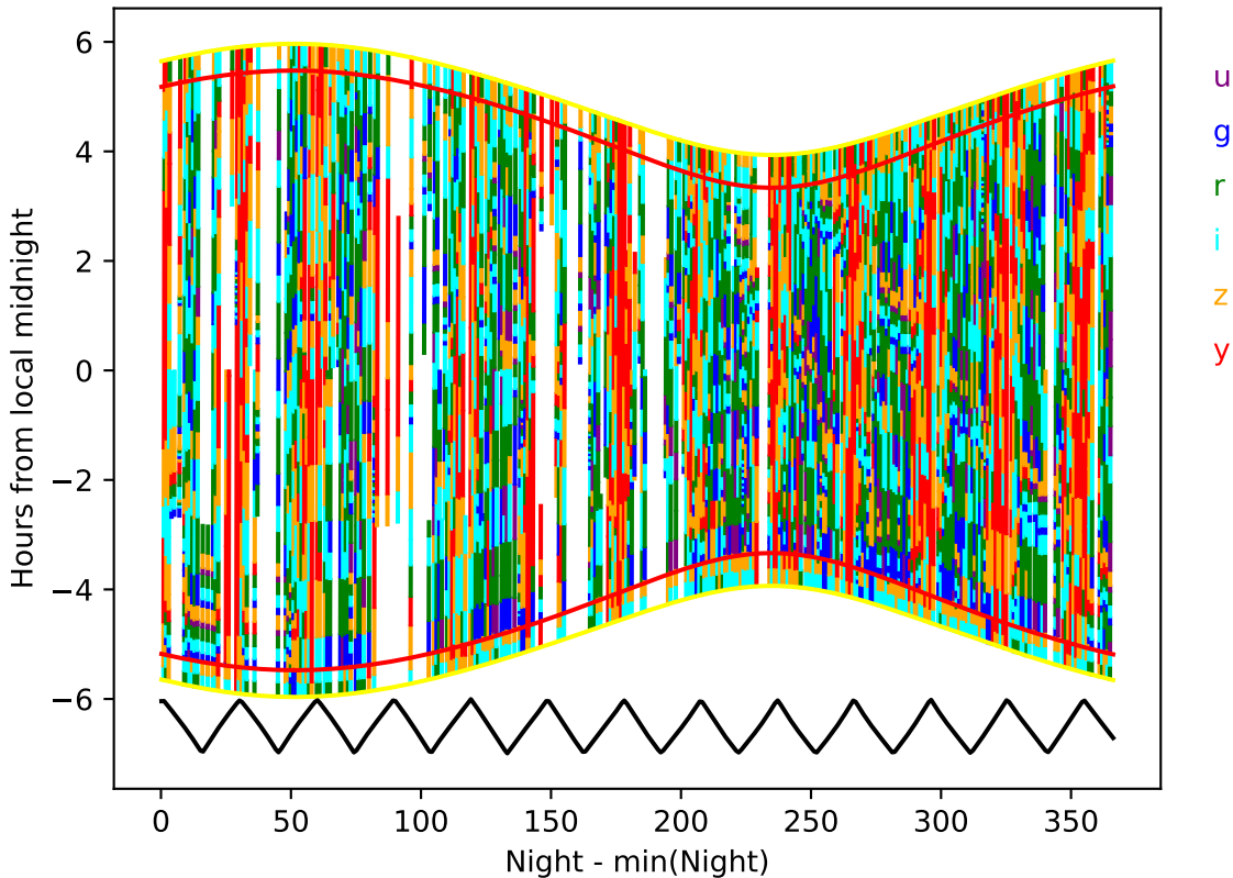
too_elab_r32_d3_griz_v3.4_10yrs year 1-2: Hourglass
