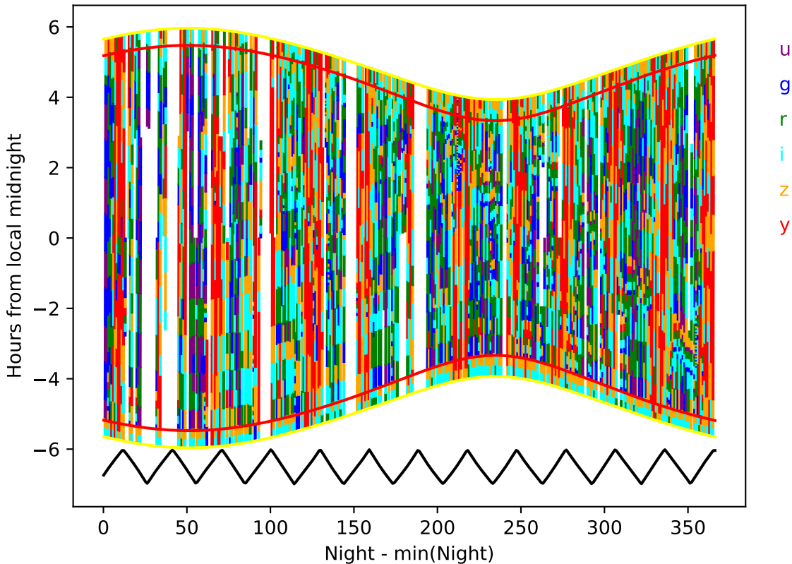
too_elab_r32_d3_griz_v3.4_10yrs year 0-1: Hourglass
