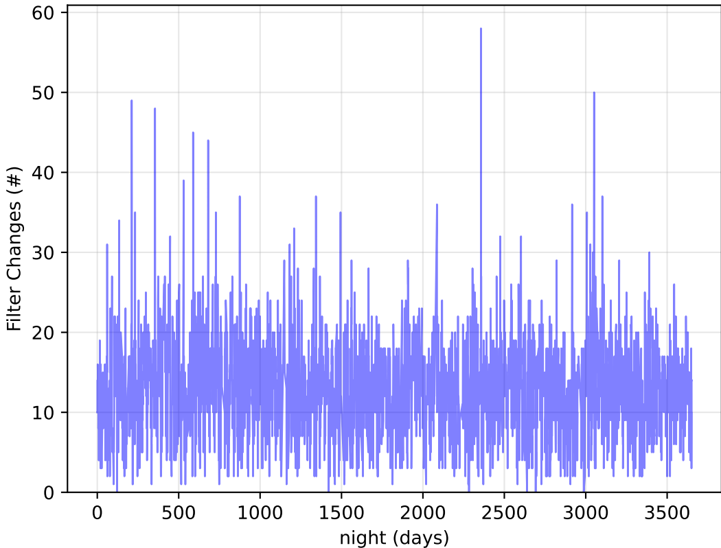
too_elab_r32_d3_griz_v3.4_10yrs : Filter Changes
