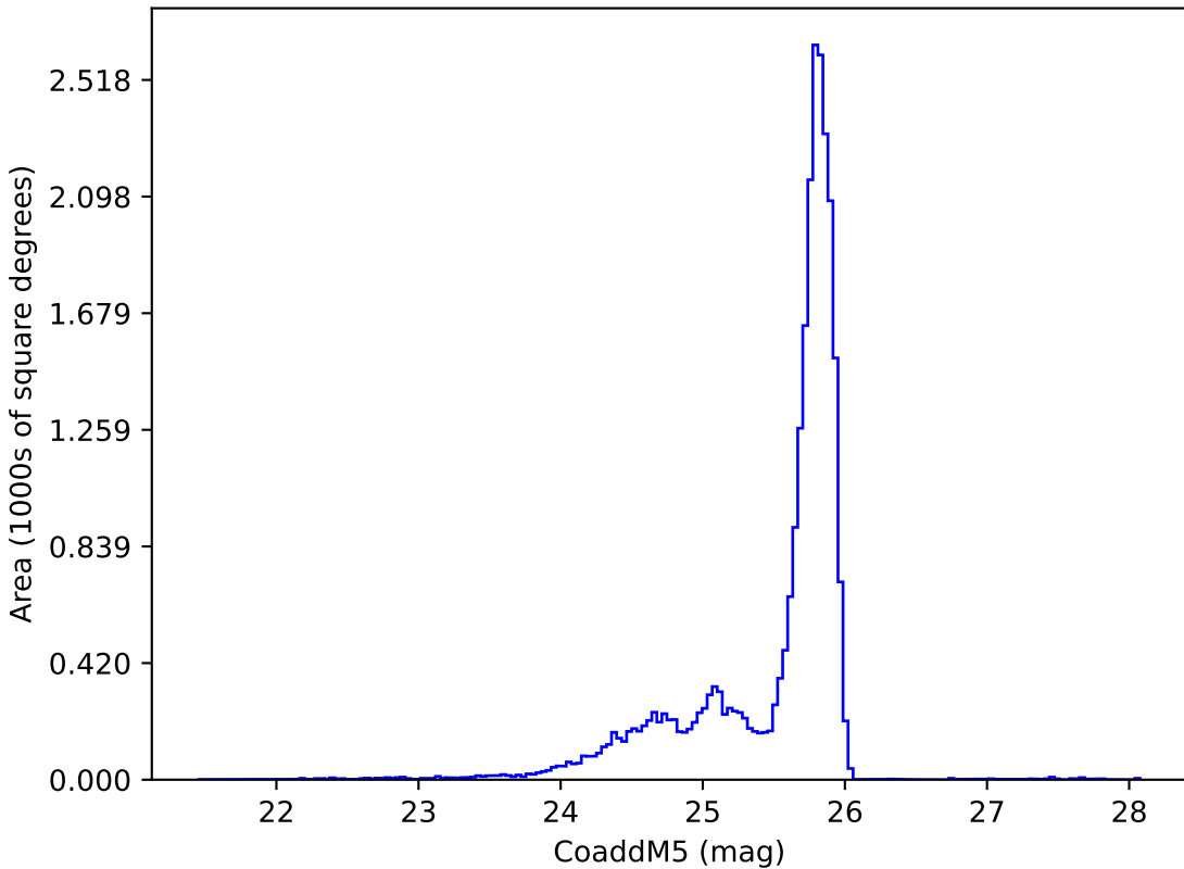
too_elab_r32_d3_griz_v3.4_10yrs z: CoaddM5
