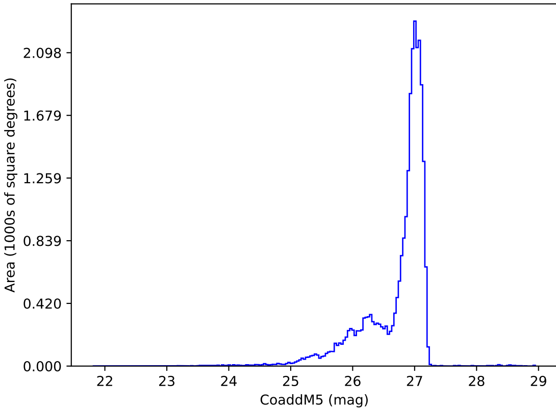
too_elab_r32_d3_griz_v3.4_10yrs r: CoaddM5
