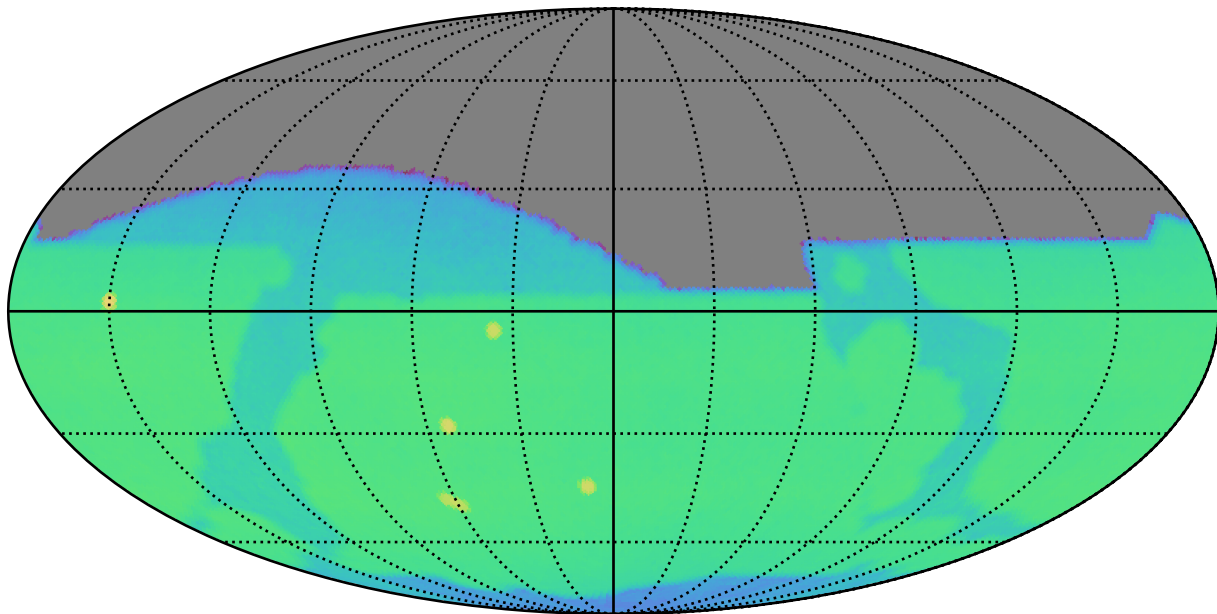
too_elab_r32_d3_griz_v3.4_10yrs i: CoaddM5
