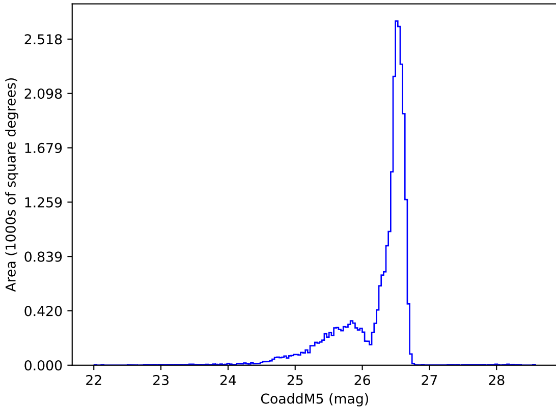
too_elab_r32_d3_griz_v3.4_10yrs i: CoaddM5
