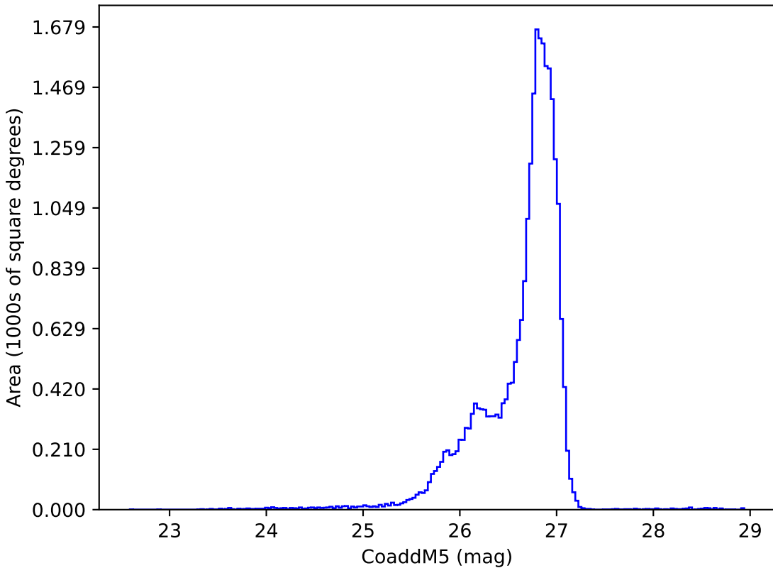
too_elab_r32_d3_griz_v3.4_10yrs g: CoaddM5
