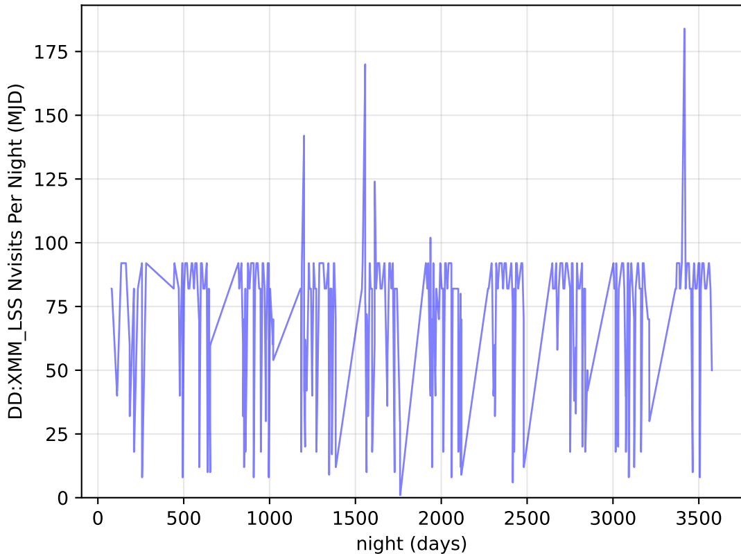
too_elab_r32_d3_griz_v3.4_10yrs all bands: DD:XMM_LSS Nvisits Per Night
