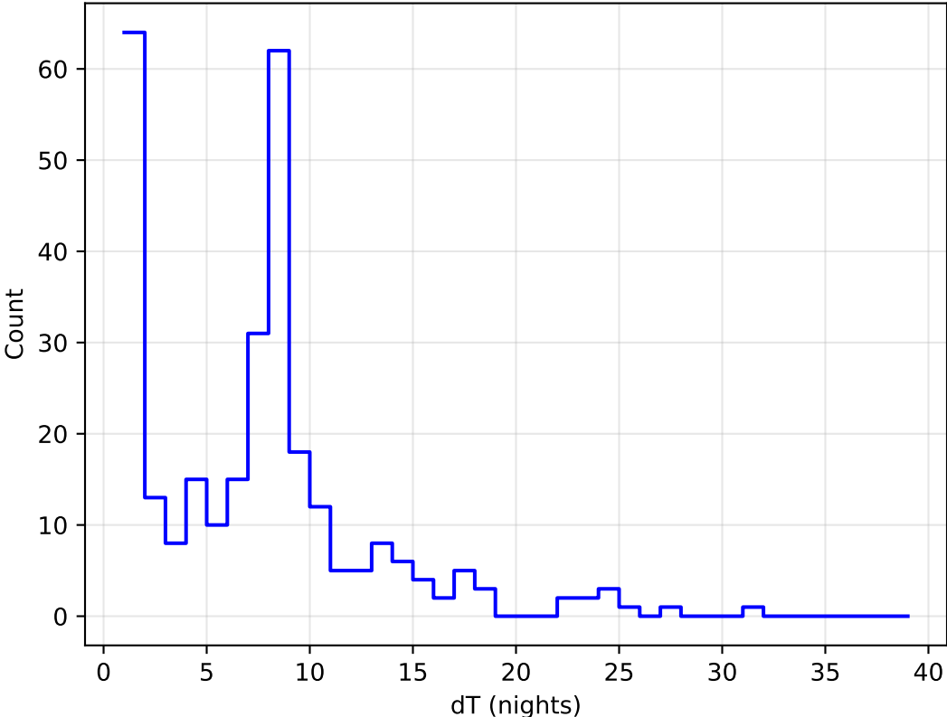
too_elab_r32_d3_griz_v3.4_10yrs all bands: DD:XMM_LSS Delta Nights Histogram
