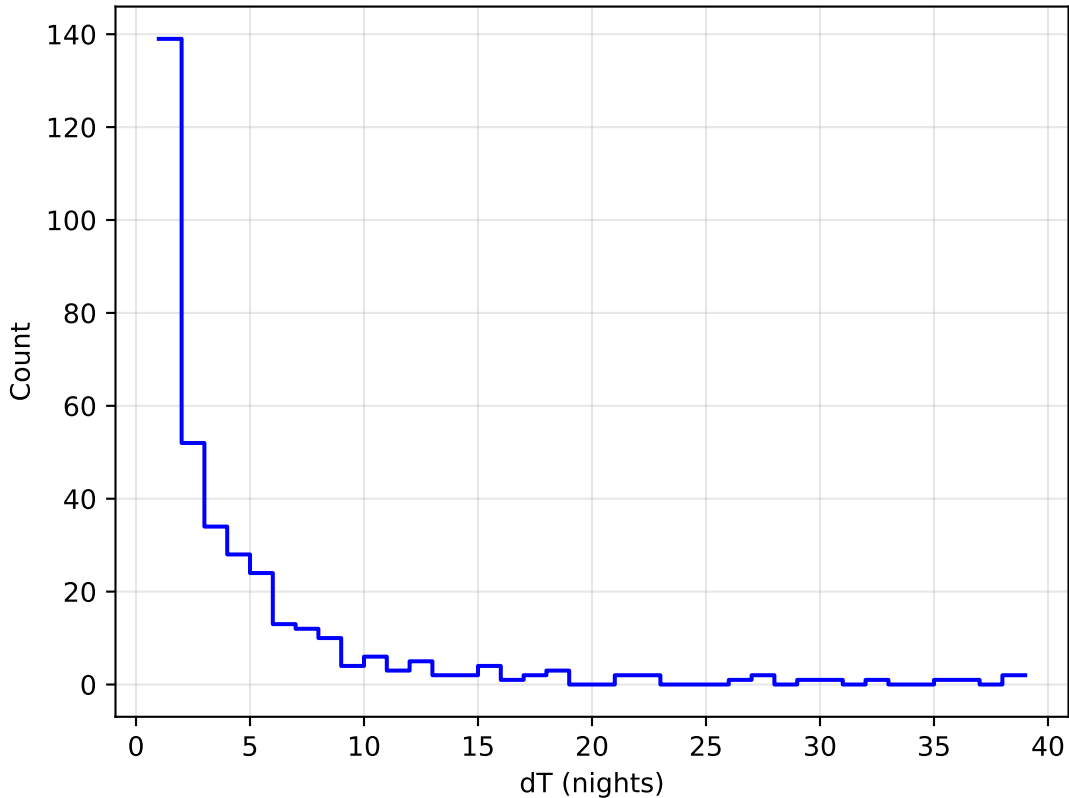
too_elab_r32_d3_griz_v3.4_10yrs all bands: DD:WFD Delta Nights Histogram
