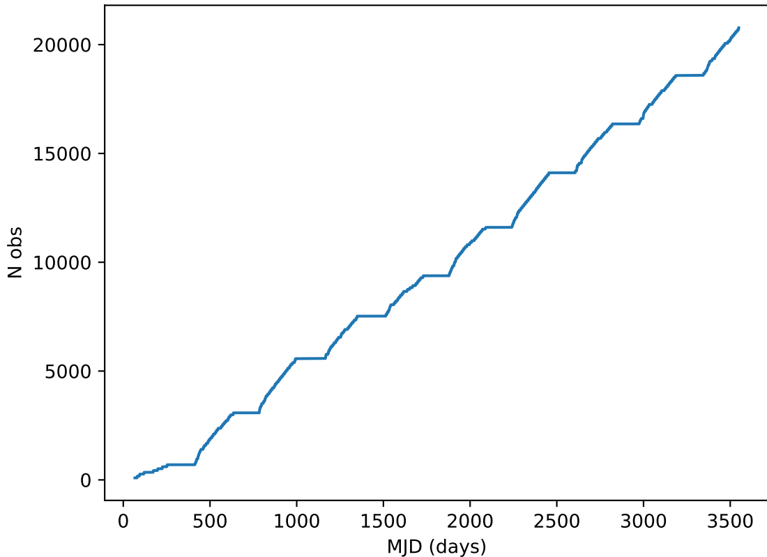
too_elab_r32_d3_griz_v3.4_10yrs all bands: DD:ELAISS1 Cumulative NVisits
