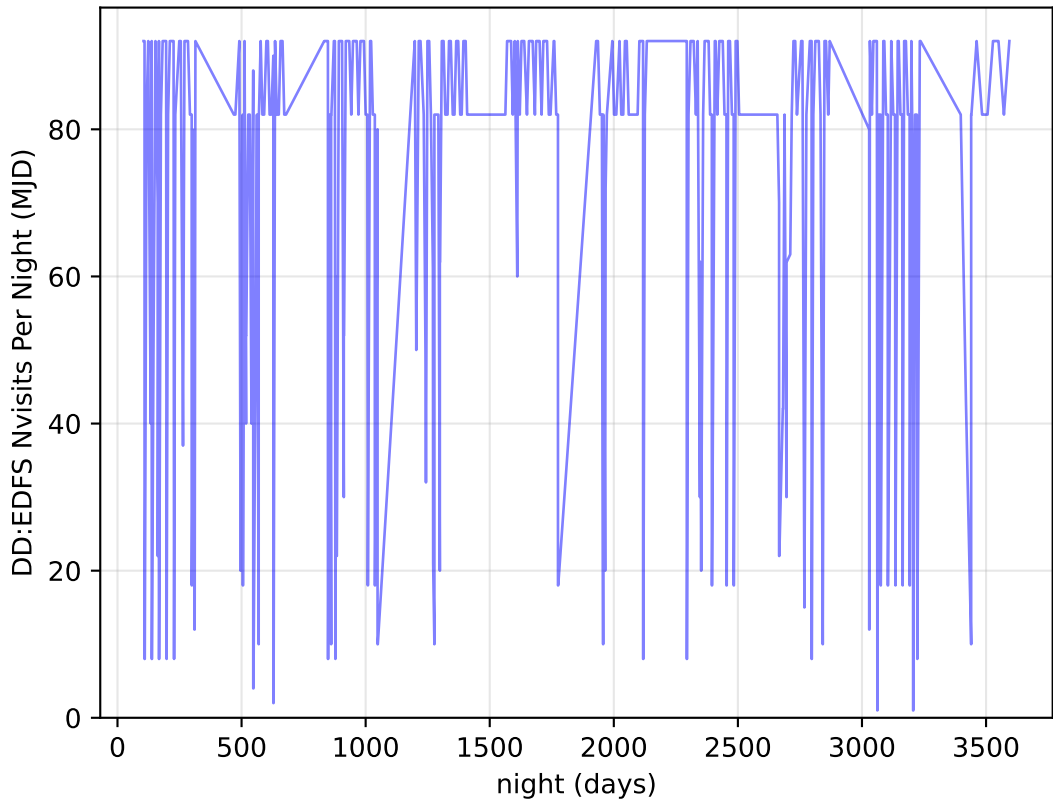
too_elab_r32_d3_griz_v3.4_10yrs all bands: DD:EDFS Nvisits Per Night
