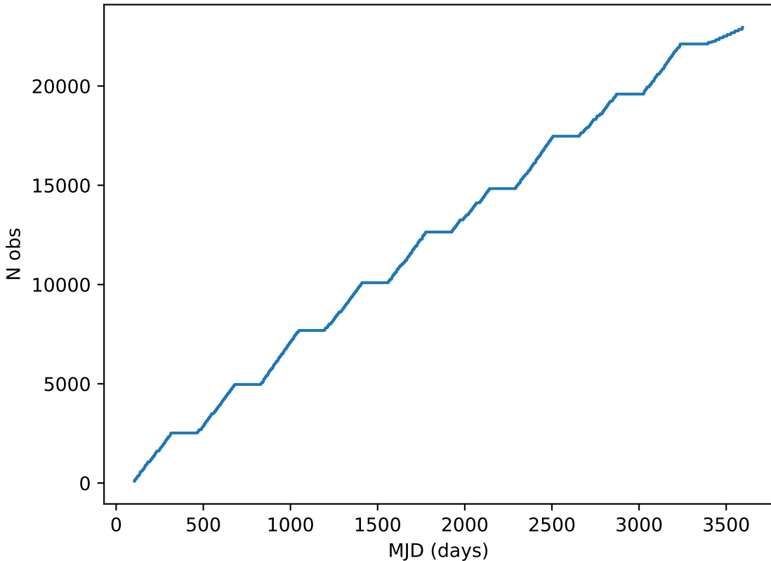
too_elab_r32_d3_griz_v3.4_10yrs all bands: DD:EDFS Cumulative NVisits
