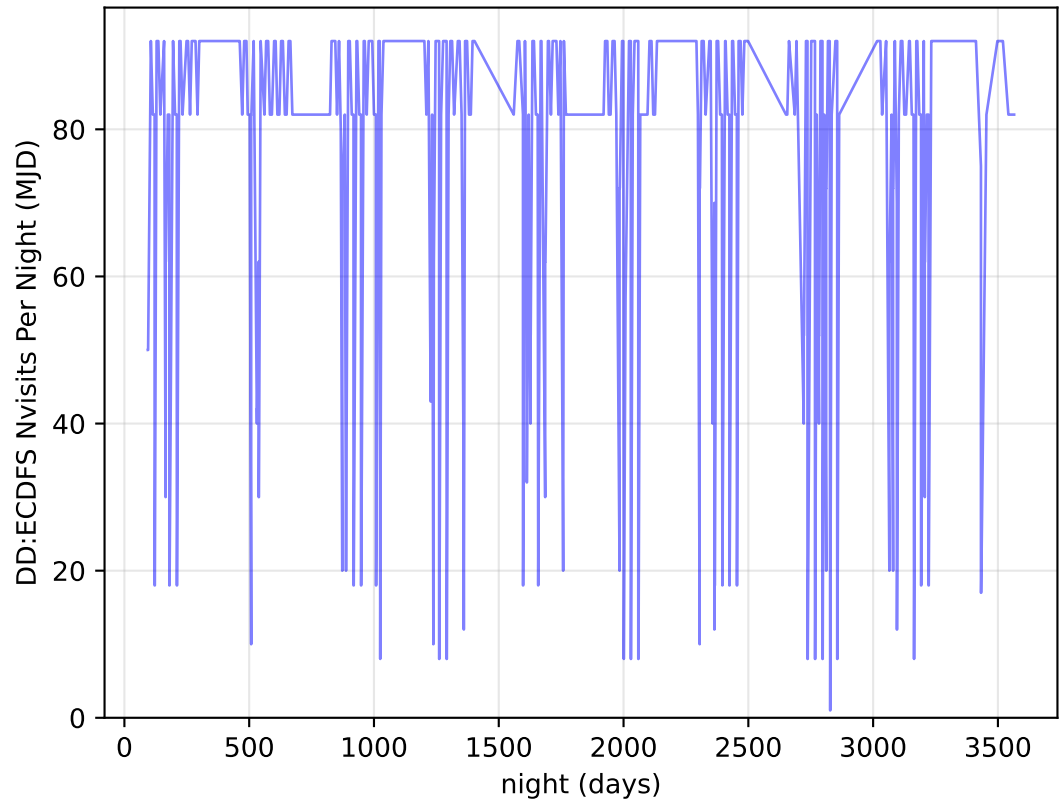
too_elab_r32_d3_griz_v3.4_10yrs all bands: DD:ECDFS Nvisits Per Night
