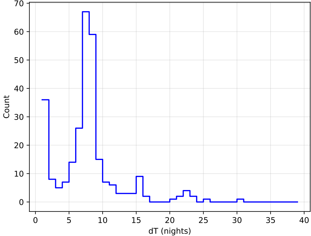
too_elab_r32_d3_griz_v3.4_10yrs all bands: DD:ECDFS Delta Nights Histogram
