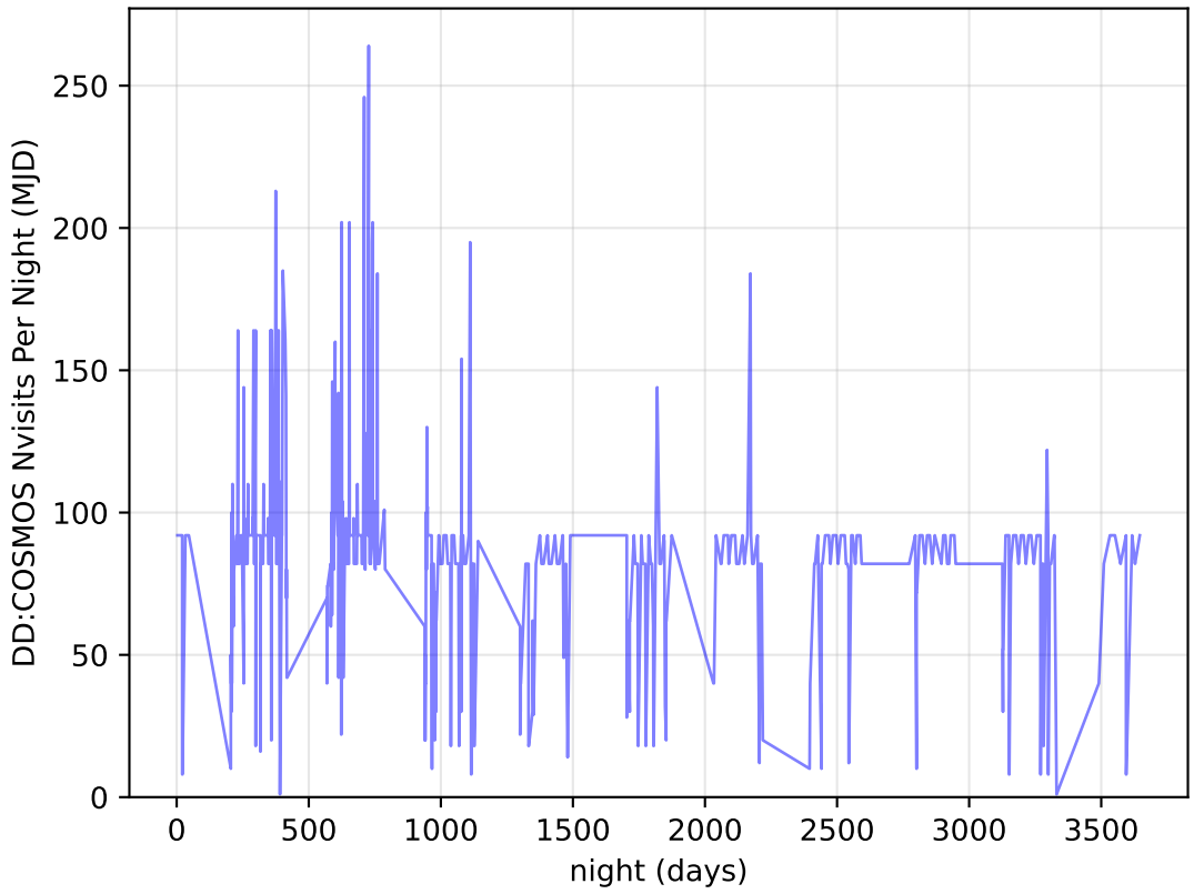
too_elab_r32_d3_griz_v3.4_10yrs all bands: DD: COSMOS Nvisits Per Night
