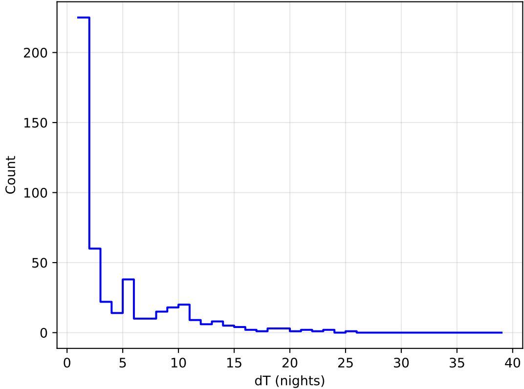
too_elab_r32_d3_griz_v3.4_10yrs all bands: DD: COSMOS Delta Nights Histogram
