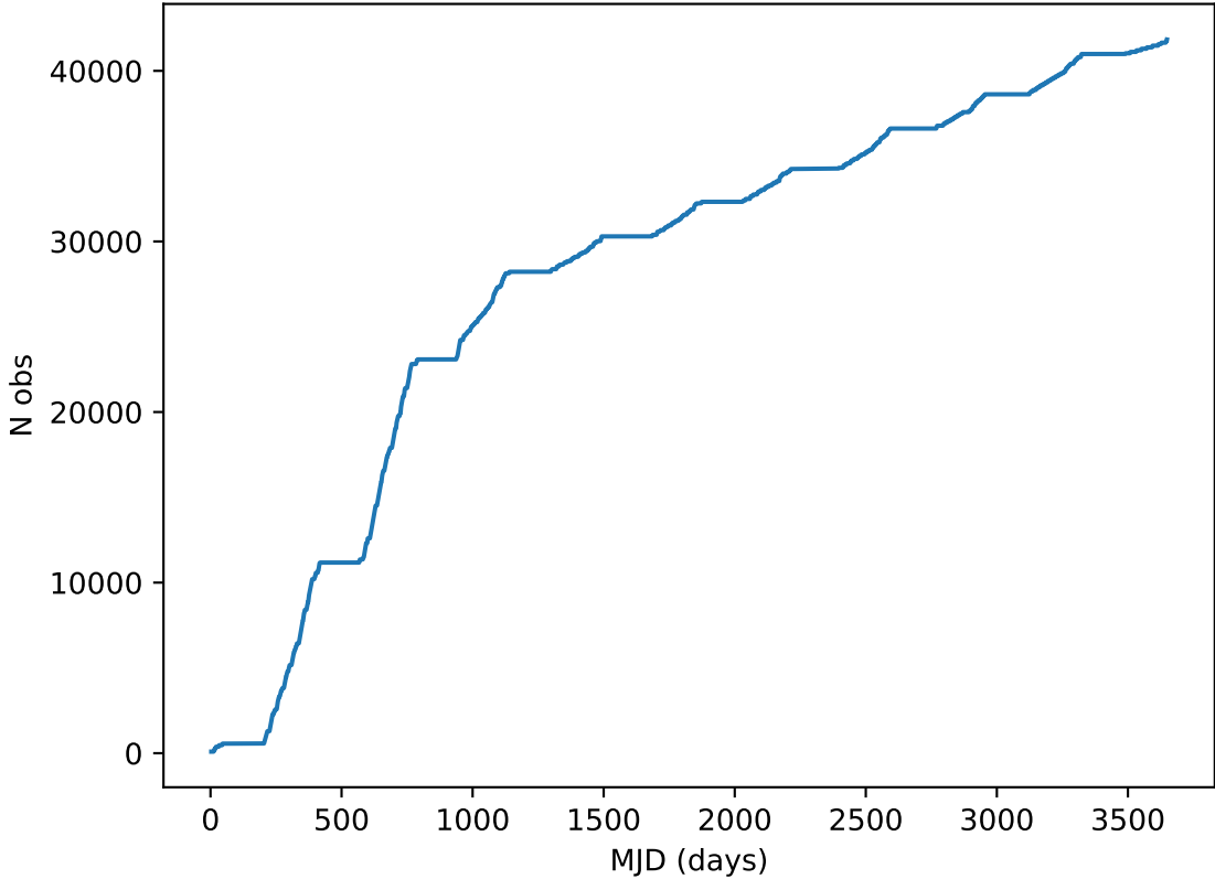
too_elab_r32_d3_griz_v3.4_10yrs all bands: DD: COSMOS Cumulative NVisits
