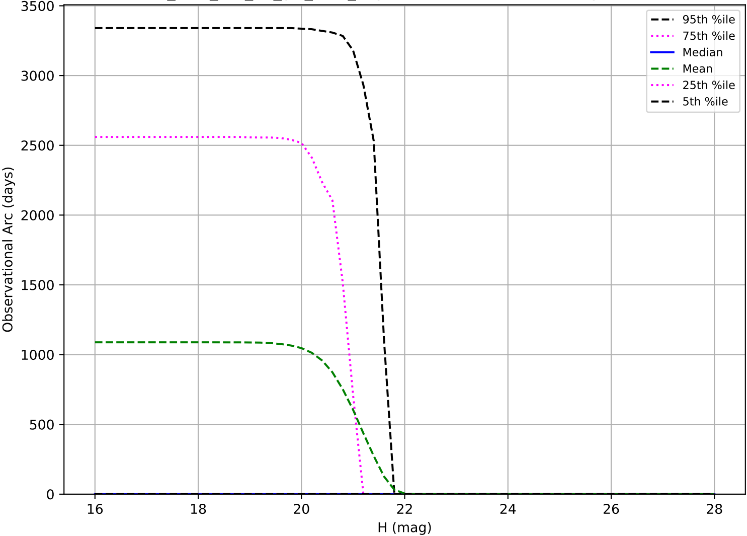
too_elab_r32_d3_giz_v3.4_10yrs: Observational Arc Length Vatira
