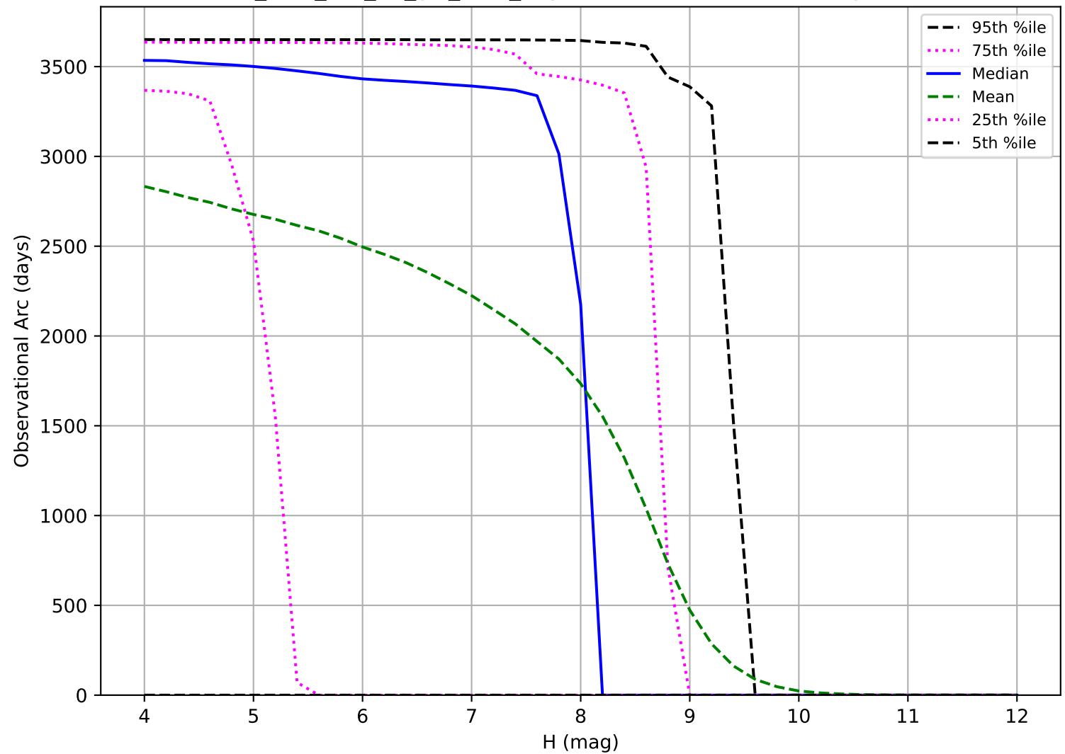
too_elab_r32_d3_giz_v3.4_10yrs: Observational Arc Length TNO
