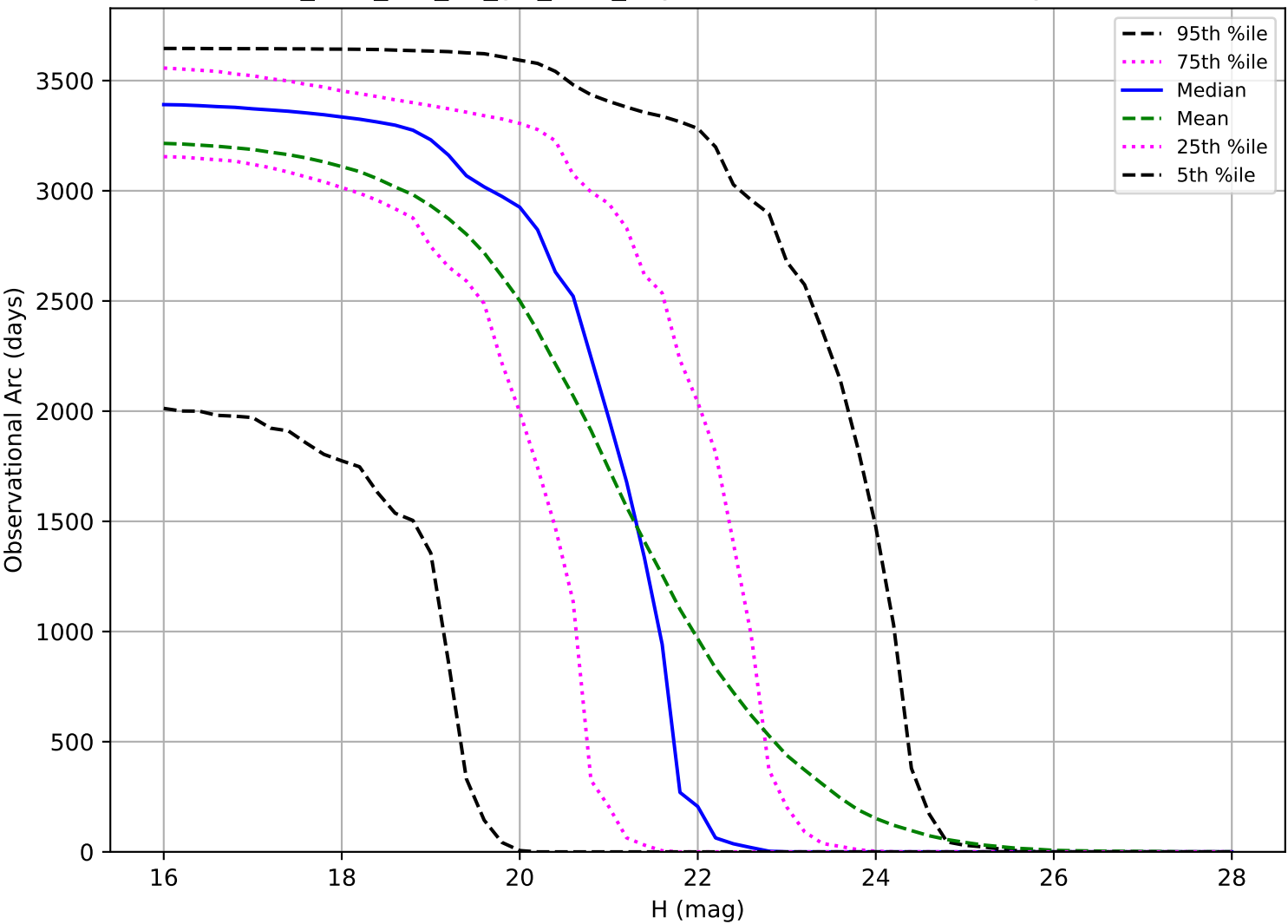
too_elab_r32_d3_giz_v3.4_10yrs: Observational Arc Length PHA
