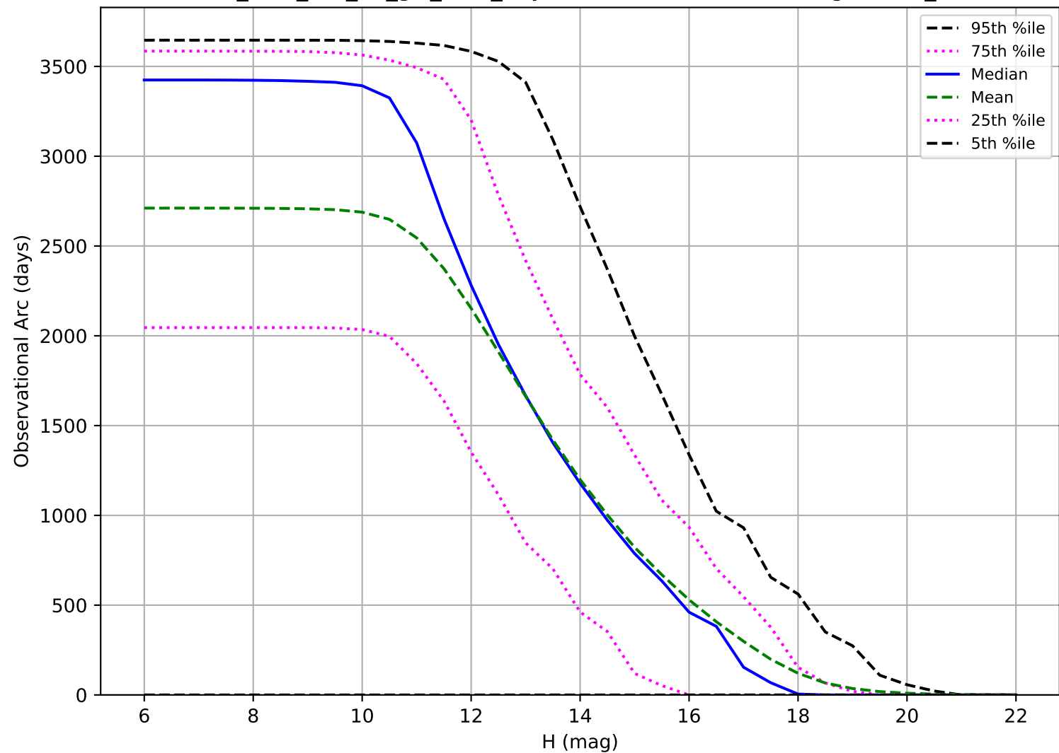
too_elab_r32_d3_giz_v3.4_10yrs: Observational Arc Length OCC_r5
