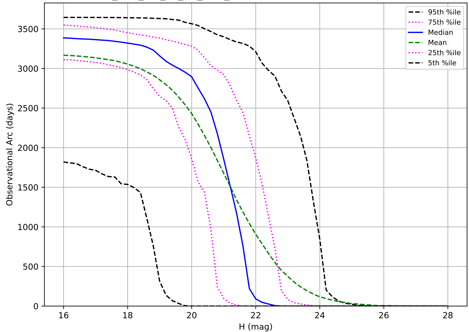
too_elab_r32_d3_giz_v3.4_10yrs: Observational Arc Length NEO
