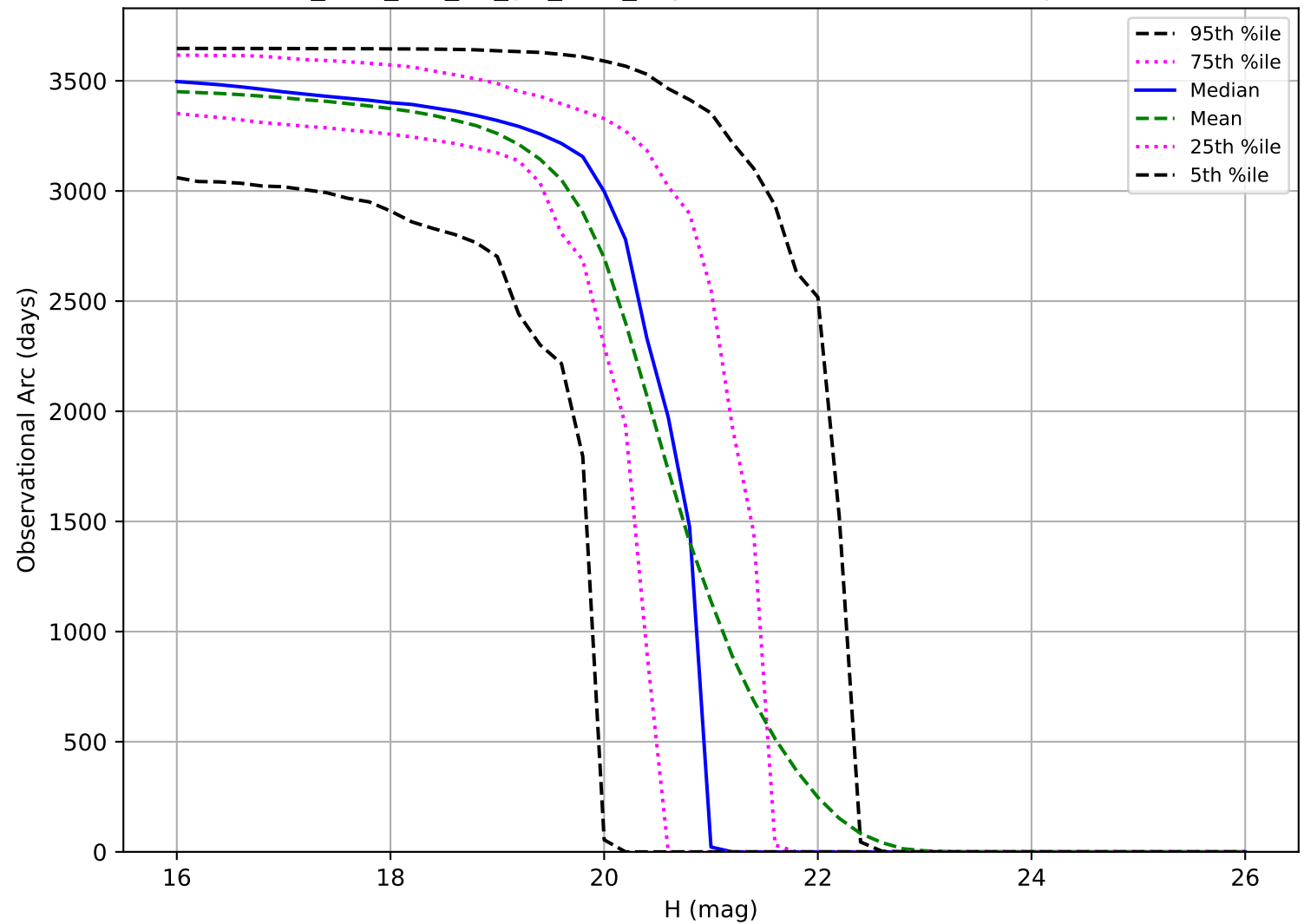
too_elab_r32_d3_giz_v3.4_10yrs: Observational Arc Length MBA
