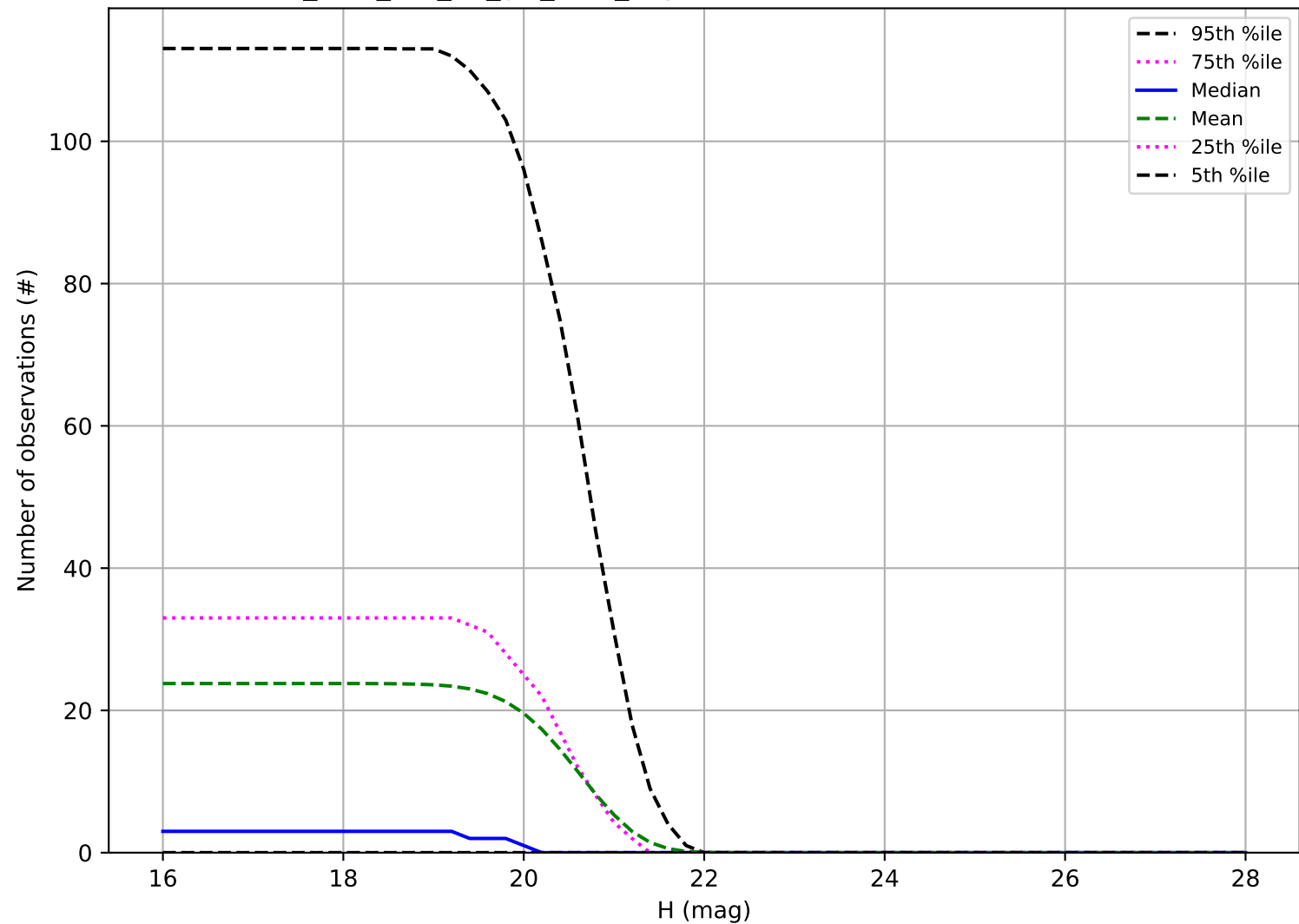
too_elab_r32_d3_giz_v3.4_10yrs: Number of observations Vatira
